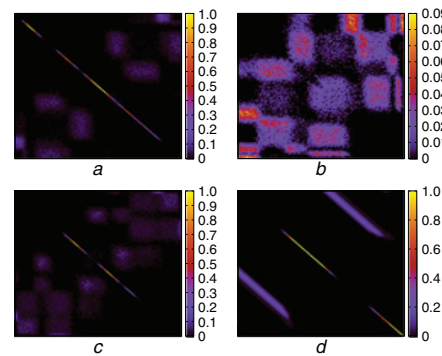
Fig. 3 Structure of quasi-optimal assignment matrix ( \Pr(X_{i,j} = 1) )
